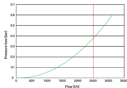
Typical pressure loss curve - DN15 R400
